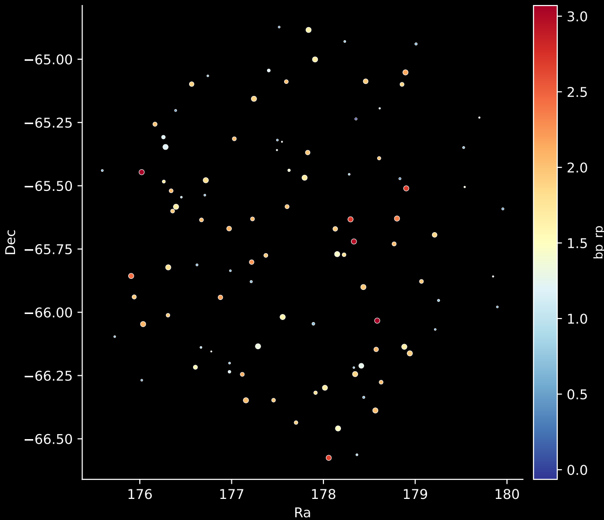
APOGEE DR17 Field: [LMC6] Stars: 101
