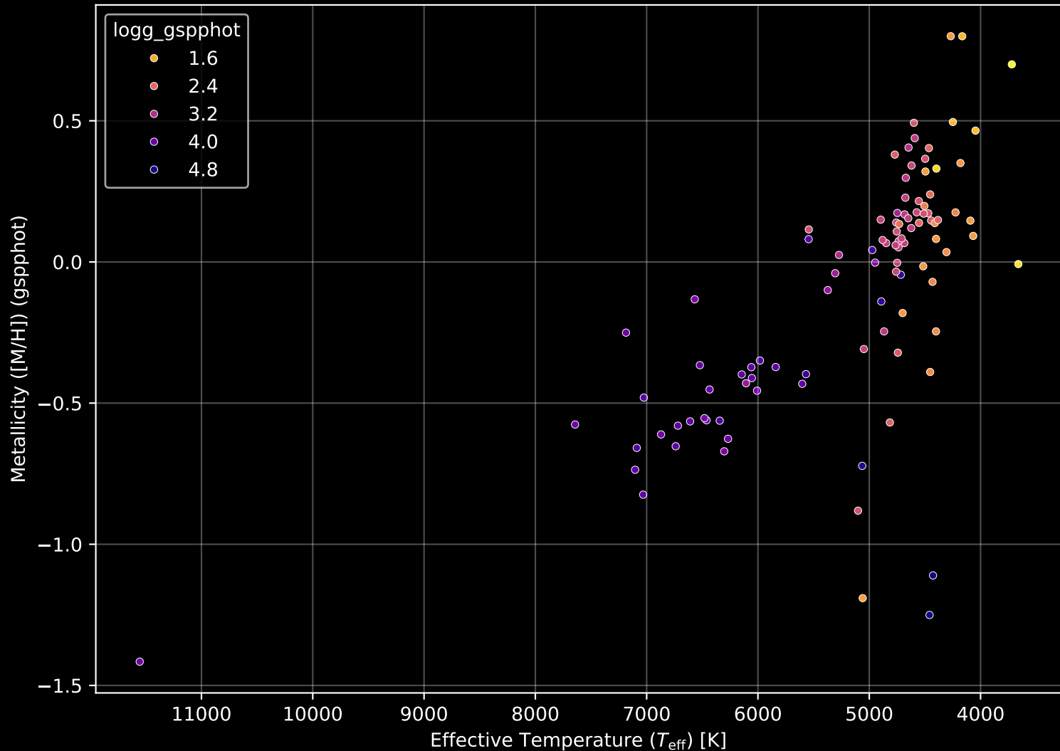
APOGEE DR17 Field: [LMC6] Stellar Population Parameters (n= 101)
