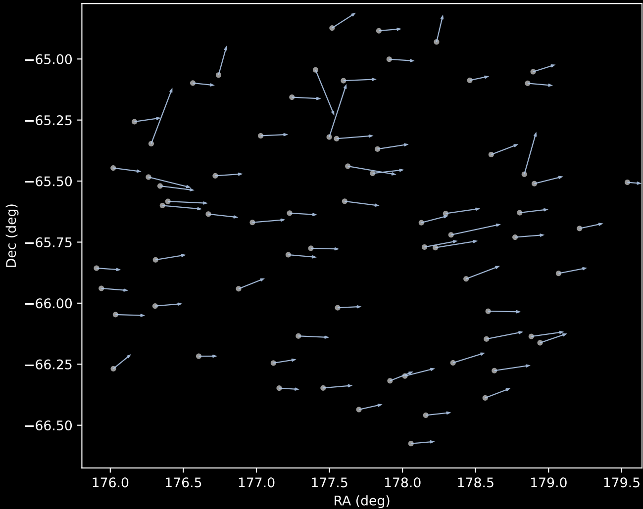
APOGEE DR17 Cluster 1 Proper Motion Vectors (n=71)
