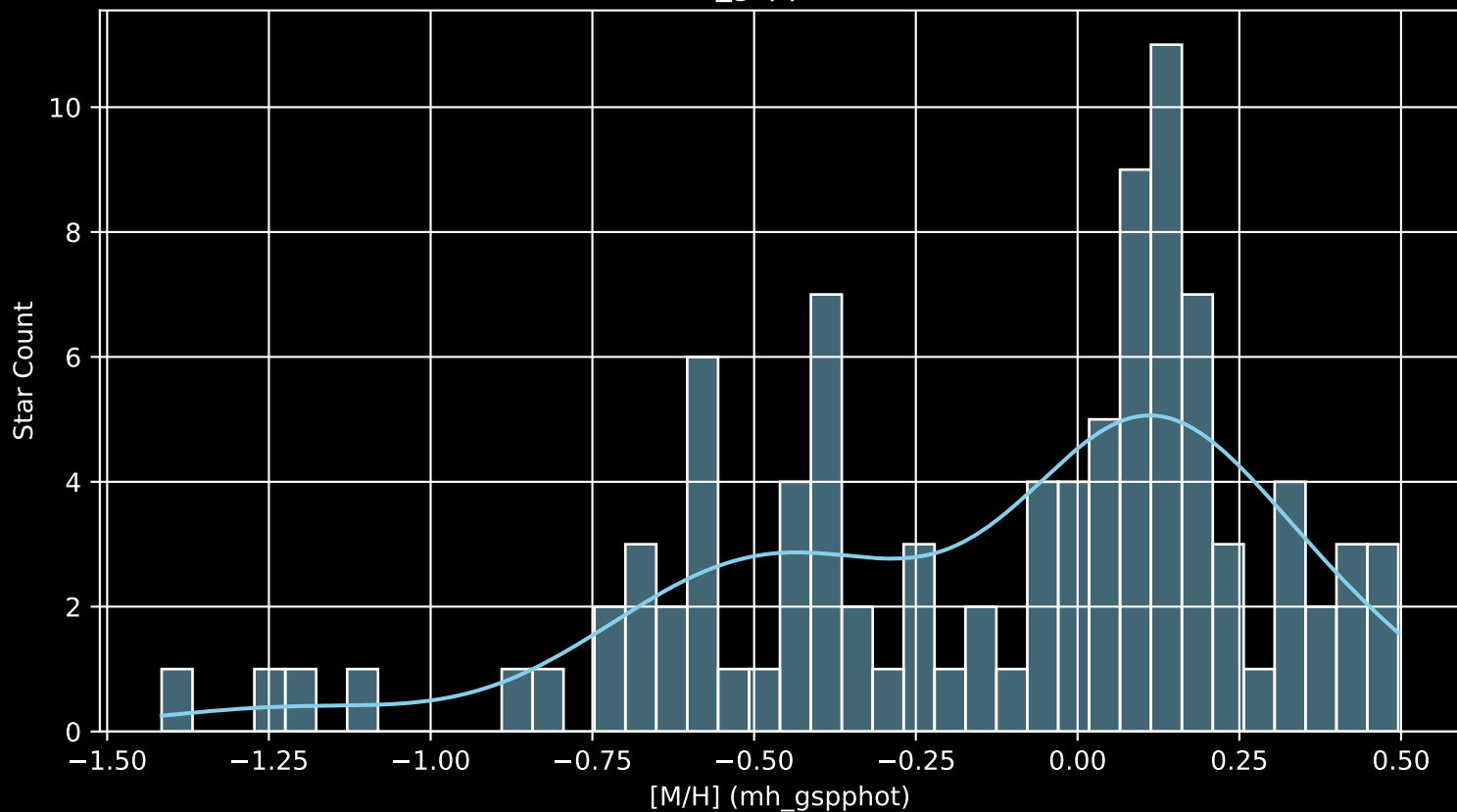
APOGEE DR17 Field: [LMC6 [M/H] (mh_gspphot) (n= 98)
