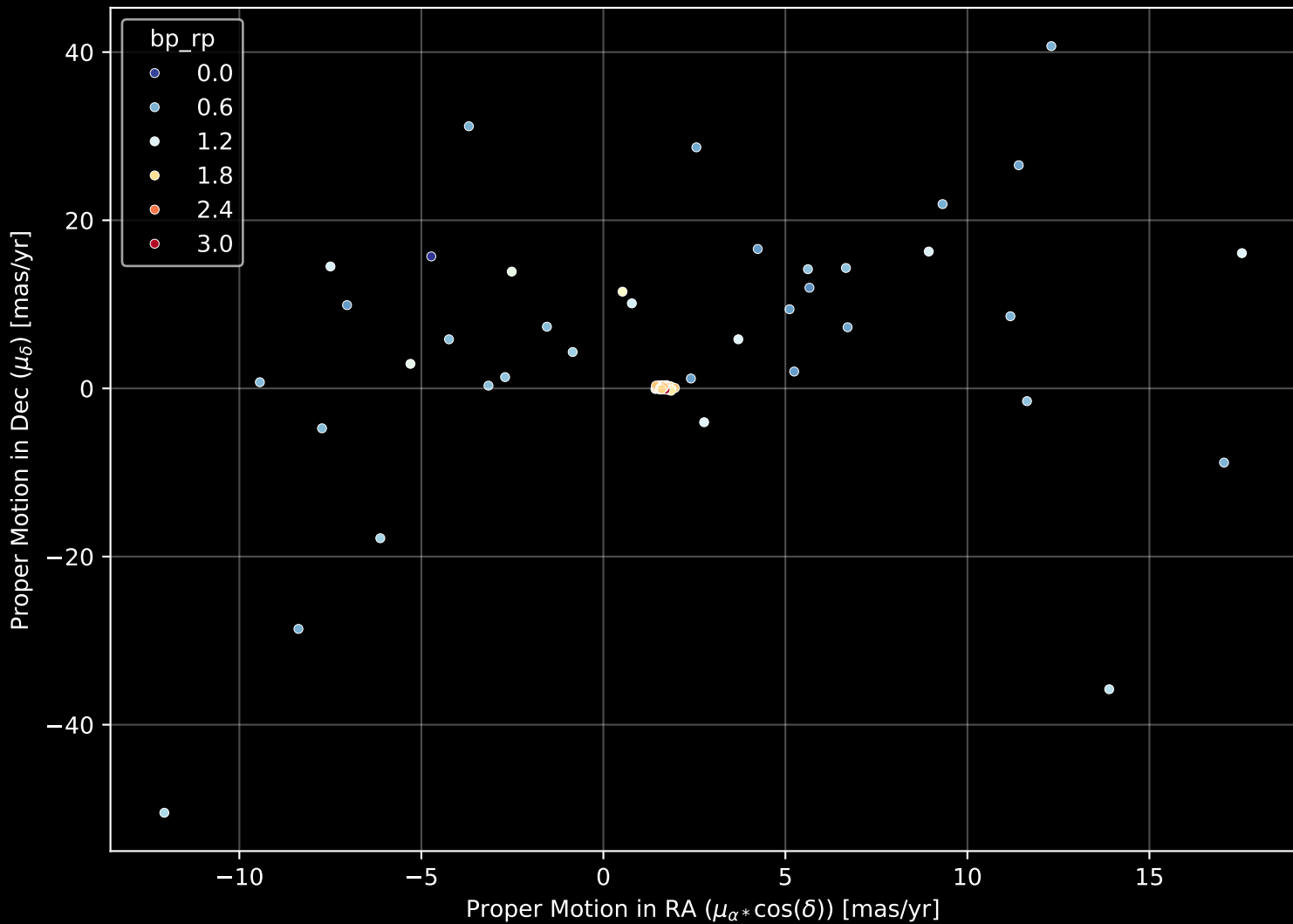
APOGEE DR17 Field: [LMC6] Proper Motion Diagram (n= 101)
