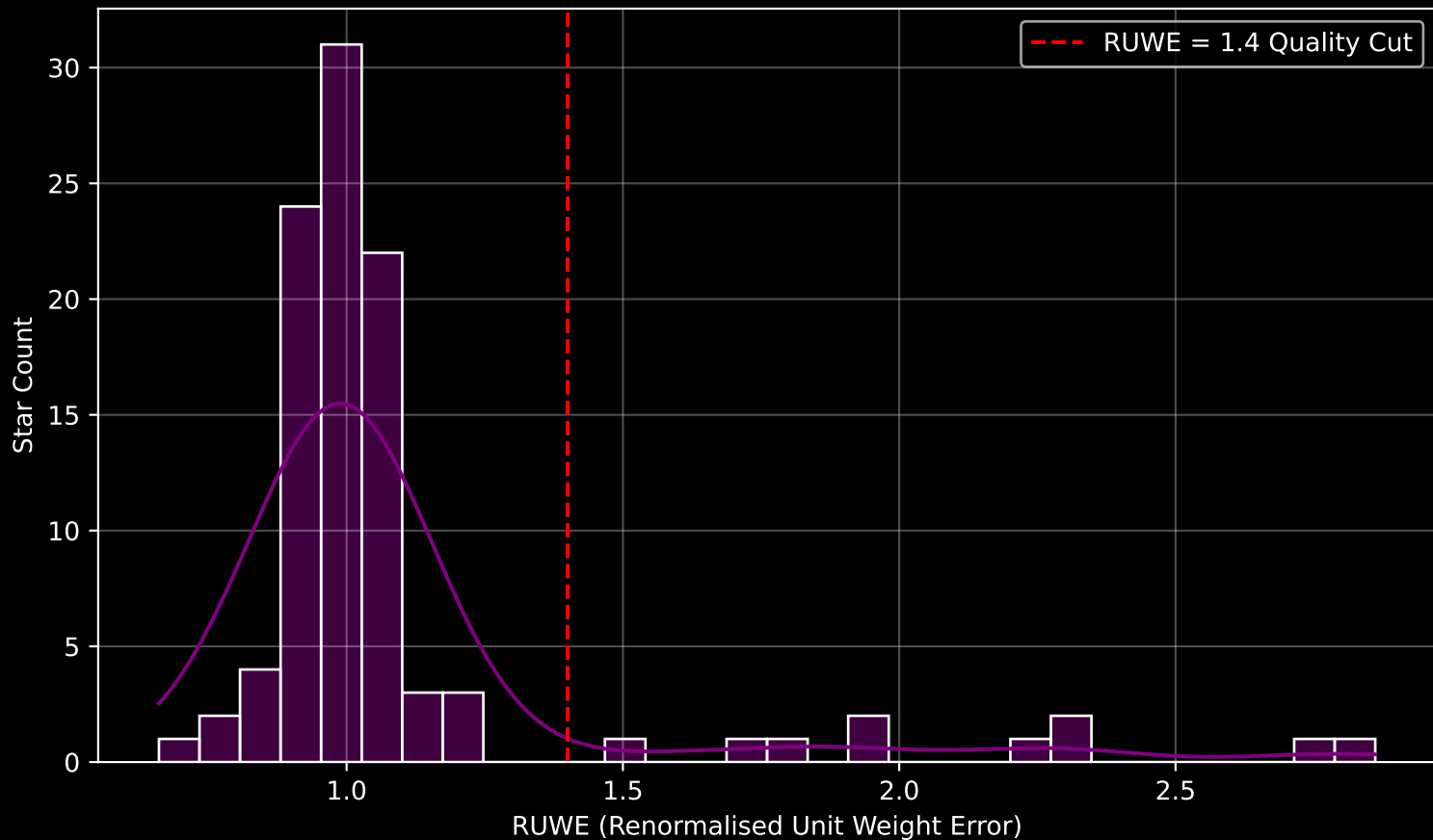
GAPOGEE DR17 Field [LMC6] RUWE Distribution (n= 100)
