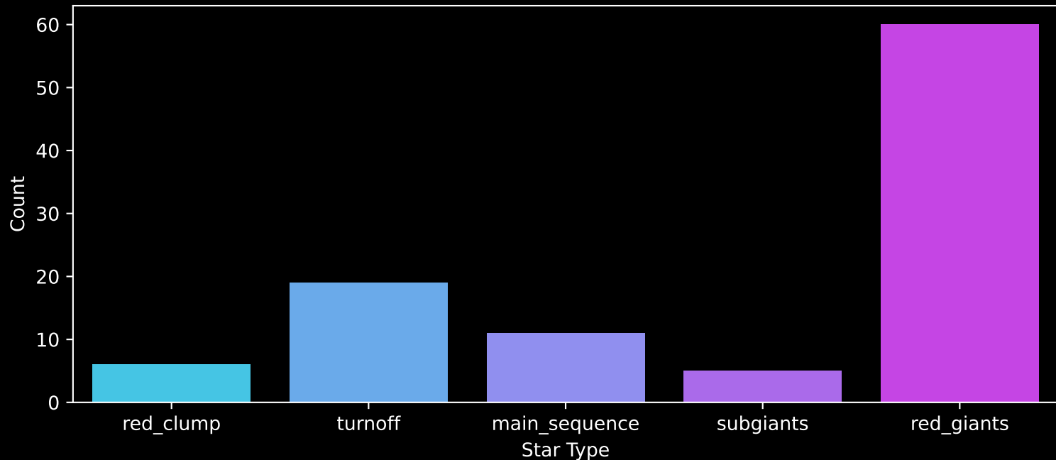
APOGEE DR17 Field: [LMC6] Count plot of Star Type
