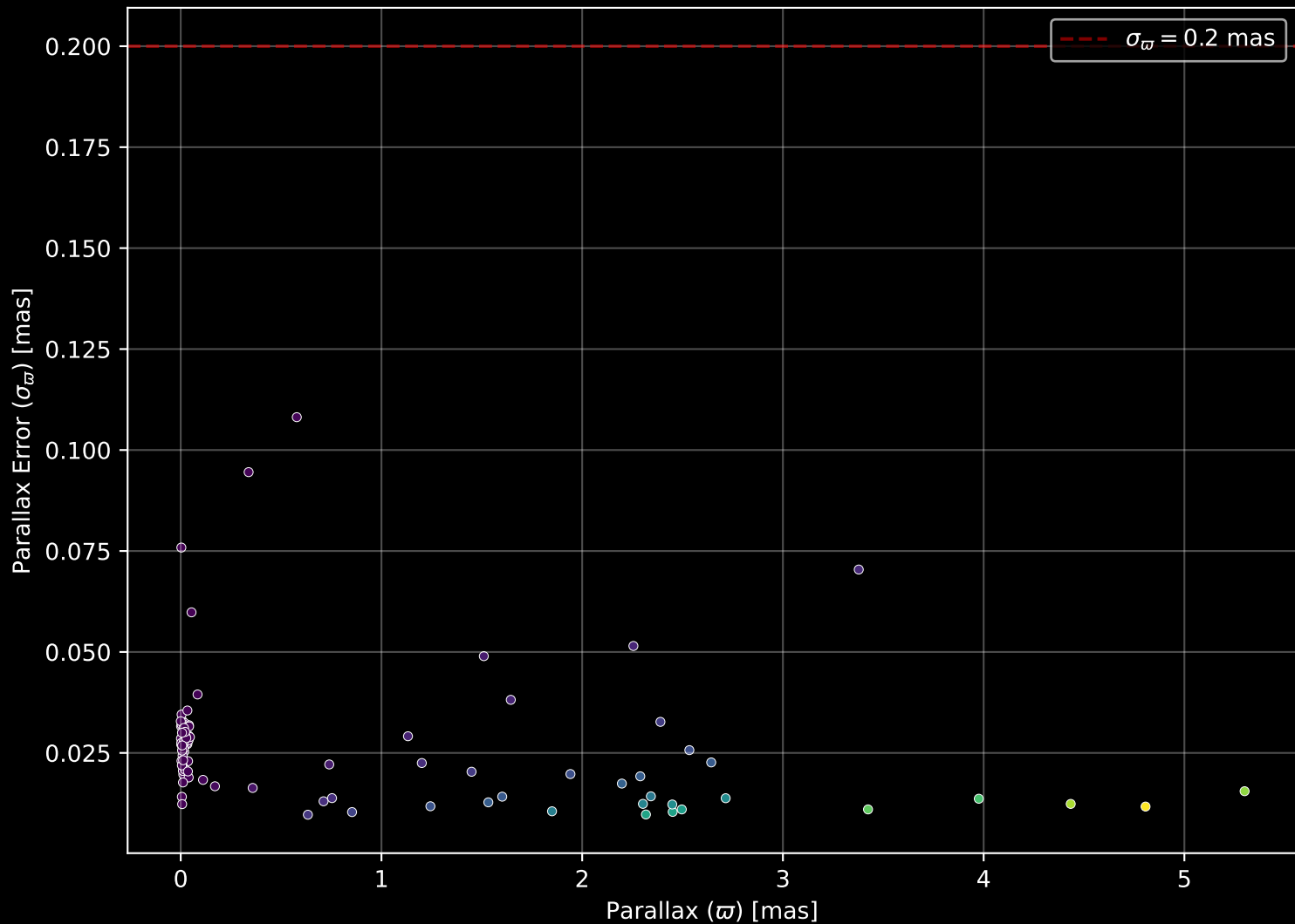
APOGEE DR17 Field: [LMC6] Parallax Quality (n= 101)
